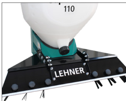
Guide plate is adjustable
